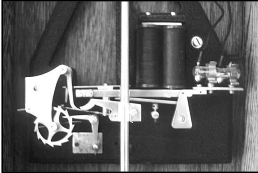
Fig. 15 Mercury switch modification
