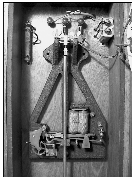
Fig. 3 Cast iron A-frame movement
